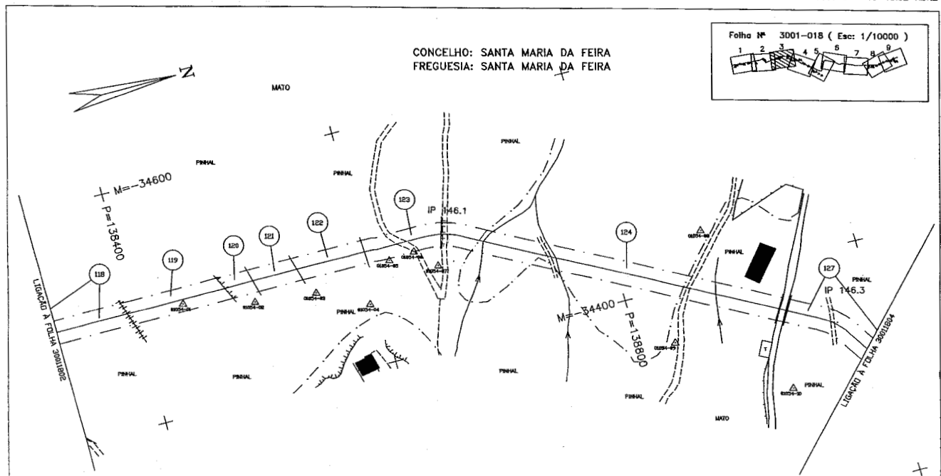
P-3001-DWG-CD-18.02-REV.2
